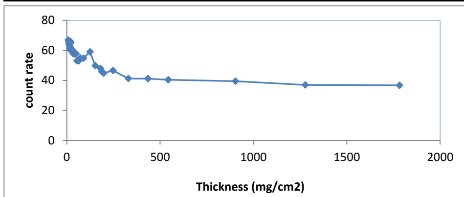
Figure 5 the attenuation of beta particle for ^{60}\text{Co}
